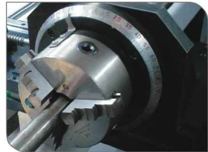
Manual feeding & turning vehicle, values readable from NC control (optional)
