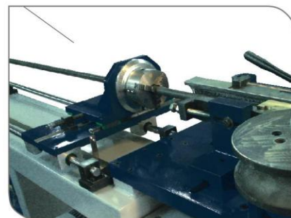
Manual feeding & turning vehicle (Optional)
